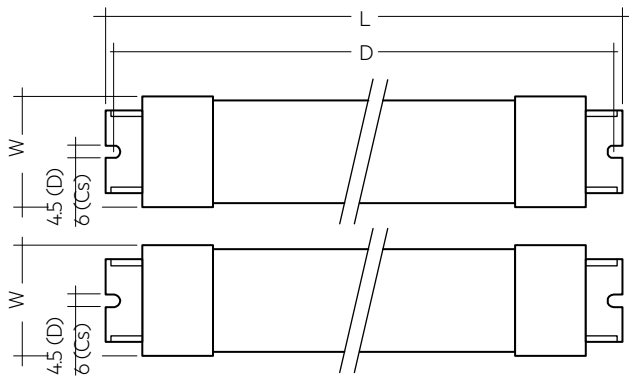
Stick + Stick; Connection: blade terminal
